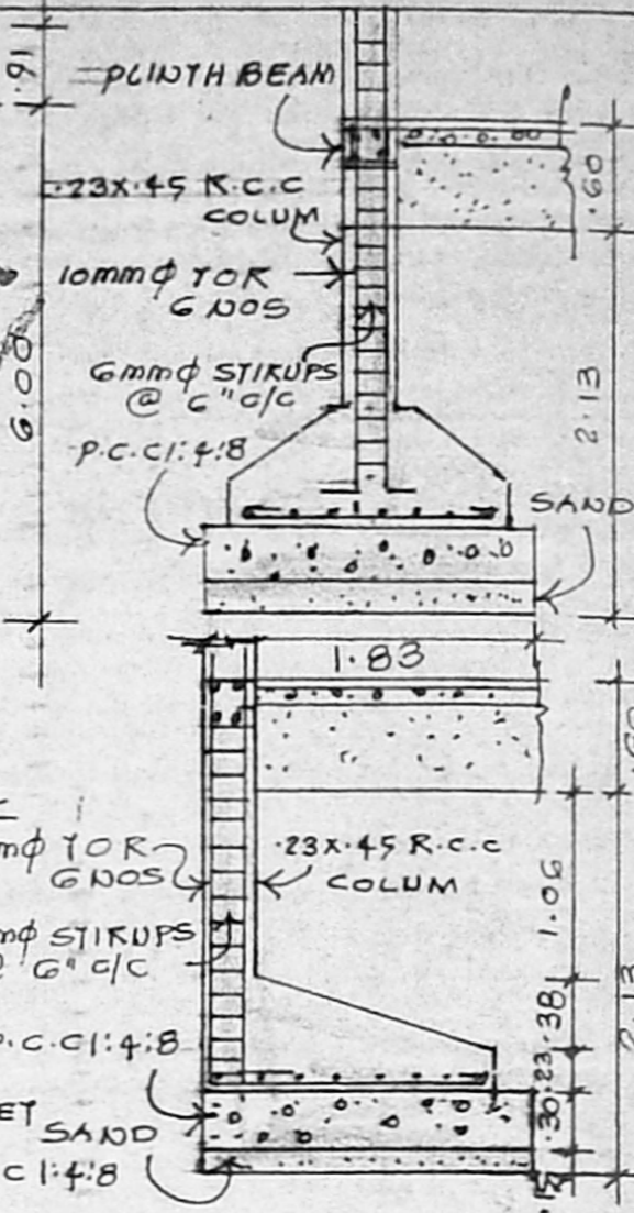
DETAIL OF FOUNDATION SCALE: 1:50
